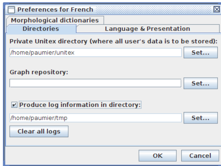
Figure 13.2: Logging configuration
