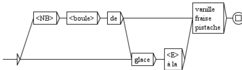
Figure 6.38: Sample graph
