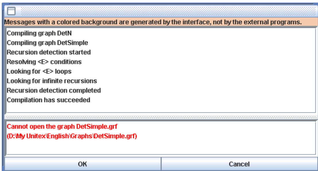
Figure 6.4: Compilation window
